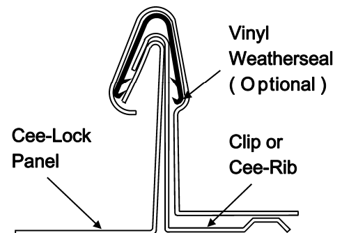
Integral Snap-Lock Seam with Patented* Vinyl Weather-seal
